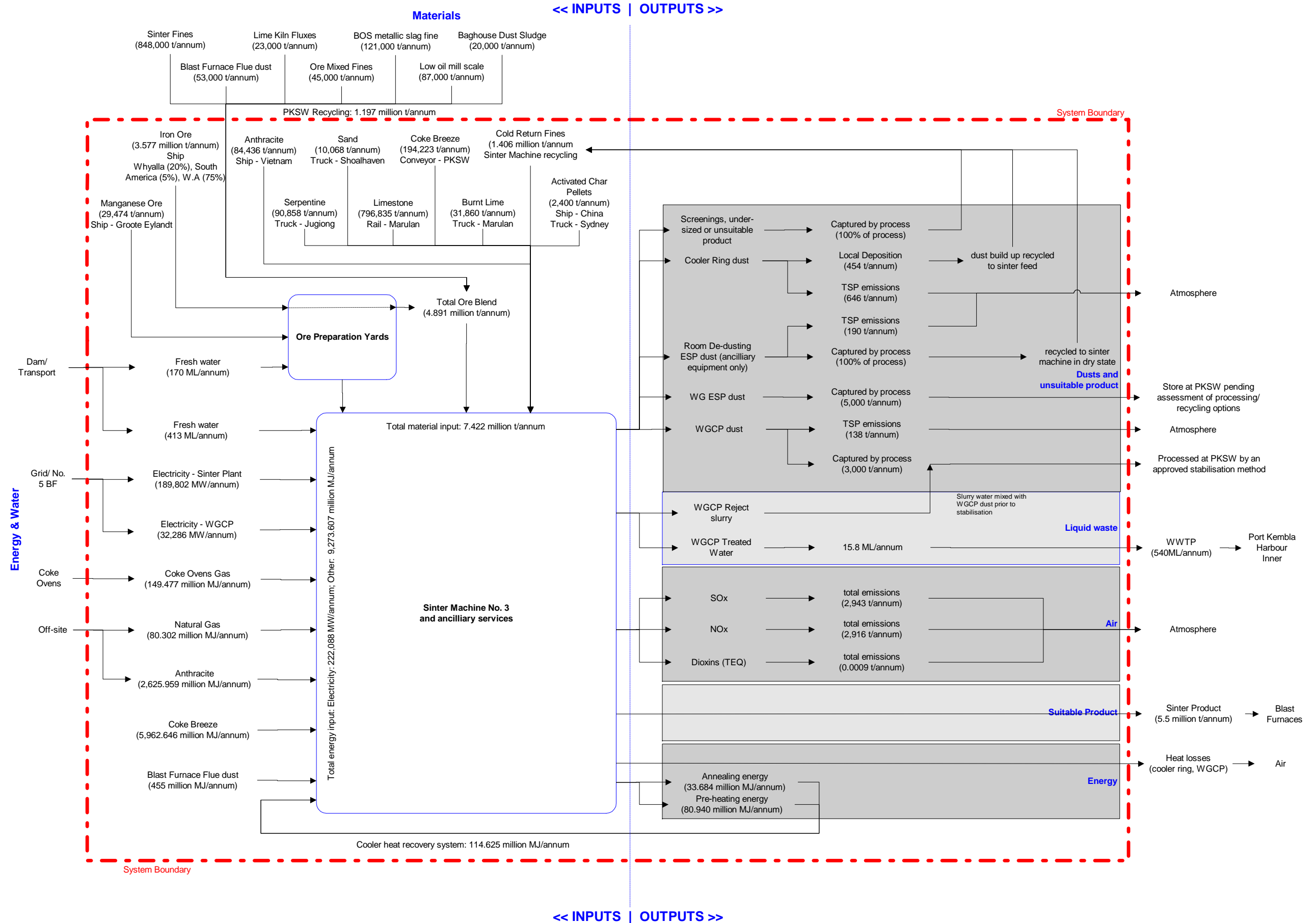
Figure G1 Sinter Plant - Current
